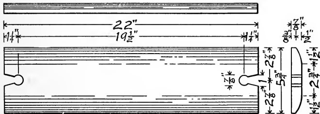
Fig. 165—Swing Board
